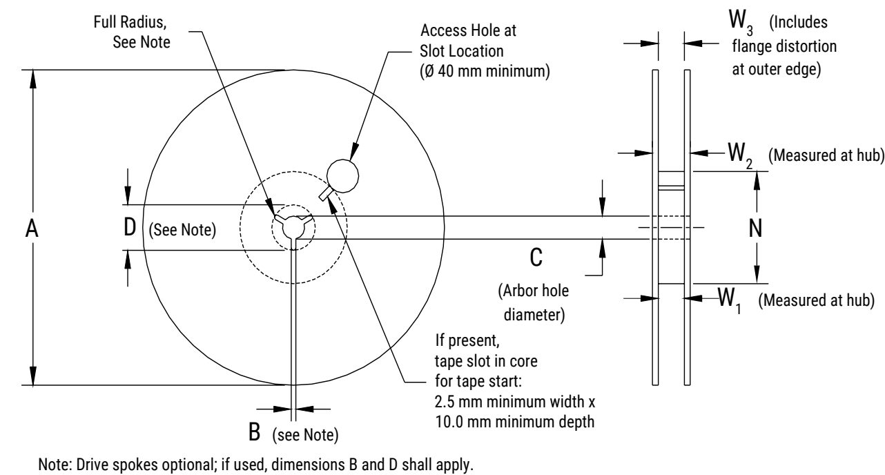
Figure 6 – Reel Dimensions
