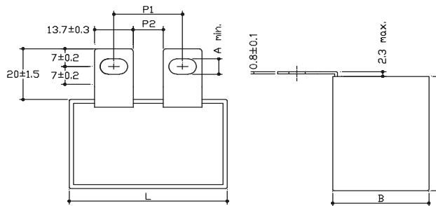
Style VN-VNM8 (for L=57,5mm only)
