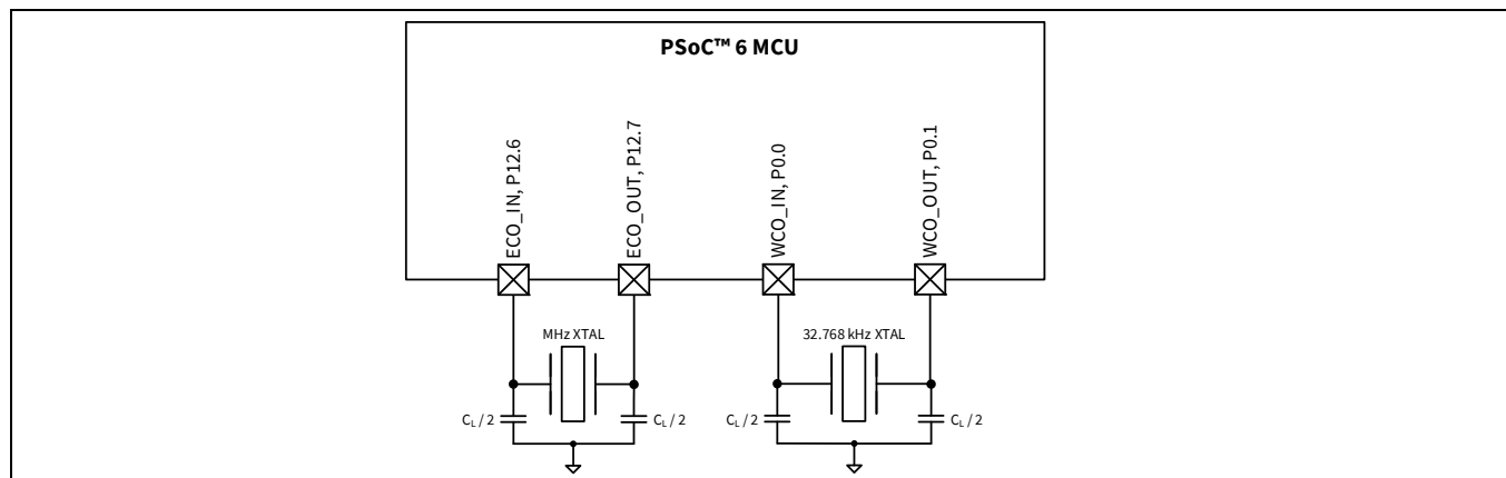
Figure 5 Oscillator circuits
