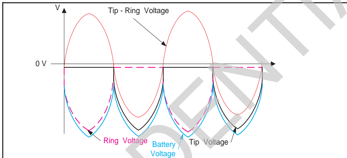
Figure 16 - Balanced Ringing with Tracking Supply
