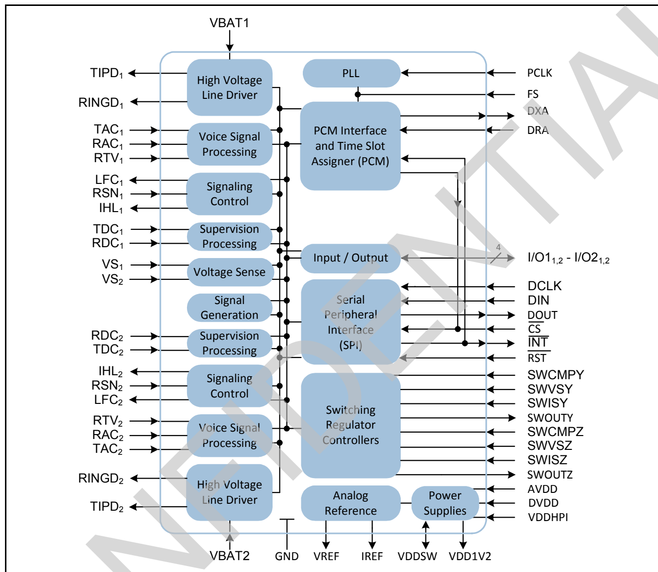
Figure 3 - Le9632 Device Block Diagram
