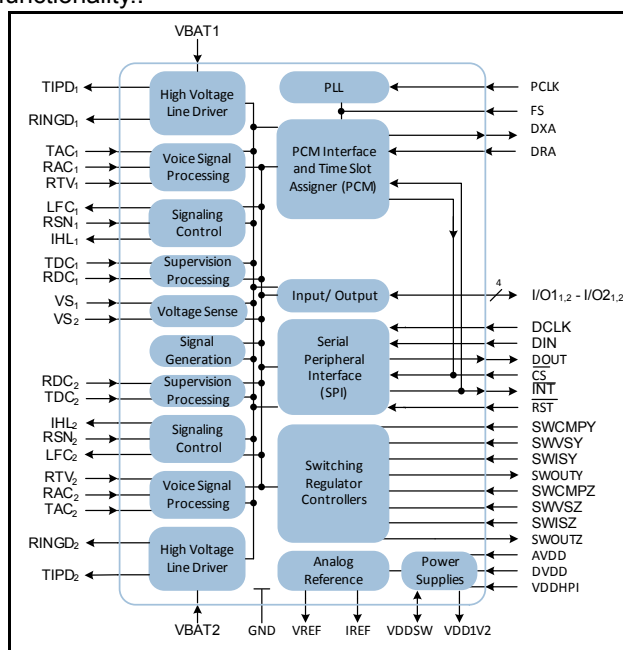
Figure 1 - Le9632 Device Block Diagram
