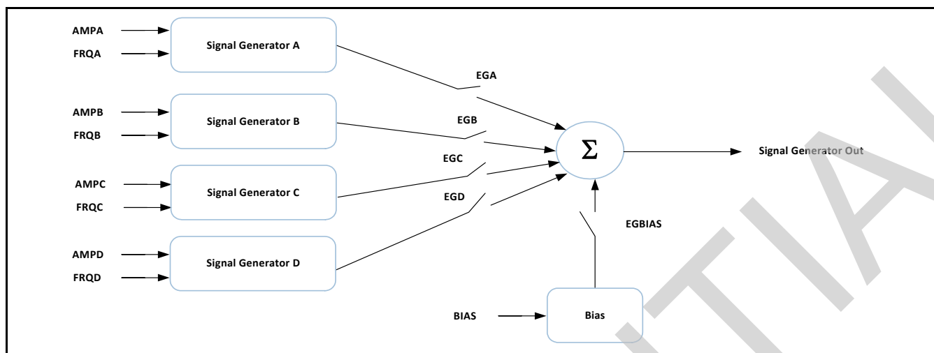
Figure 12 - Multi-Tone Generation
