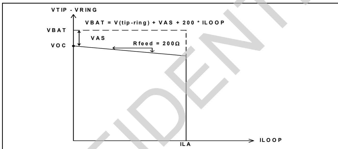
Figure 15 - Active State I / V Characteristic
