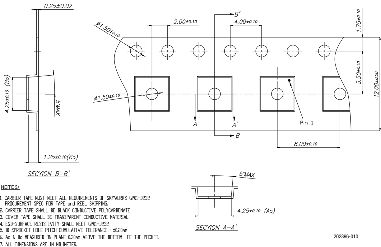
Figure 10. SE5516A Tape and Reel Dimensions
