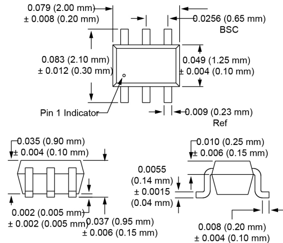
Figure 9. SC-88 Package Dimension Drawing
