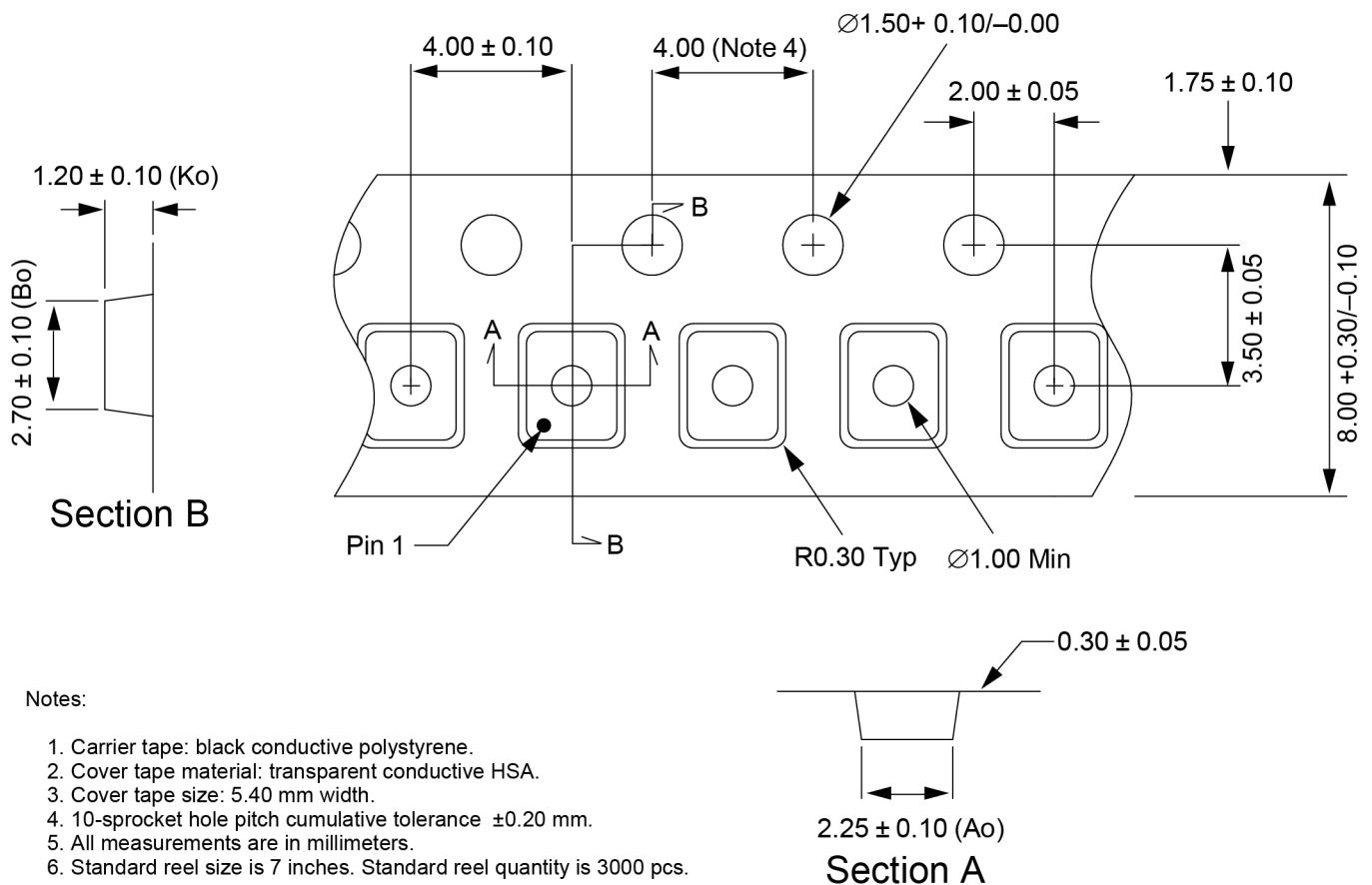
Figure 10. SC-88 Tape and Reel Dimensions
