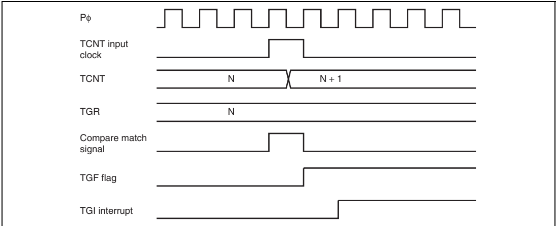
Figure 14.38 TGI Interrupt Timing (Compare Match)
