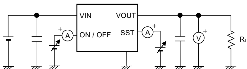
Figure 22 Test Circuit 9
