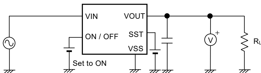
Figure 23 Test Circuit 10
