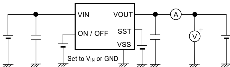
Figure 21 Test Circuit 8
