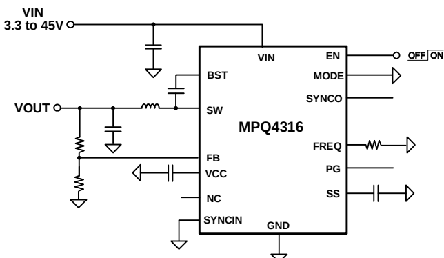
Figure 1: Output Adjustable Version
