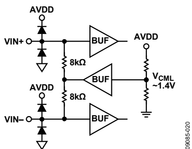
Figure 14. Analog Inputs ( V_{CML} \approx 1.4V )
