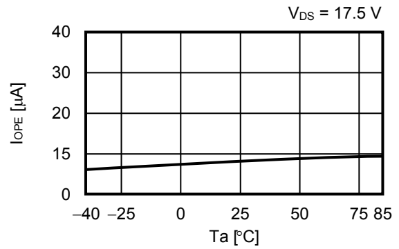
1.2 I_{OPE} vs. T_a
