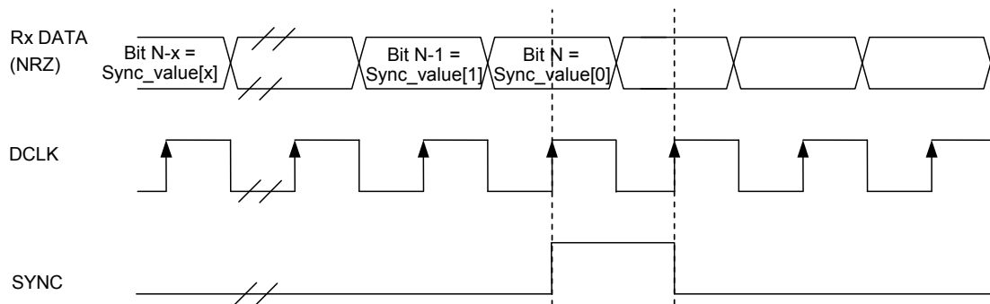
Figure 33: Sync Word Recognition
