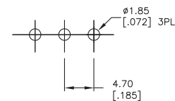
P.C. MOUNTING
