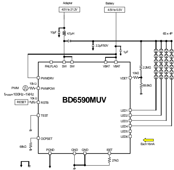
Figure 27. 6series × 4parallel, LED current 16mA, Switching frequency 1250kHz setting example Power control PWM application
