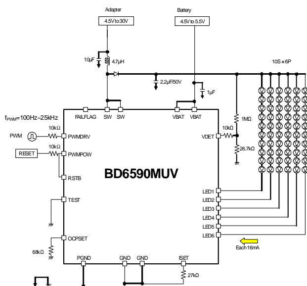
Figure 22. 10series \times 6parallel, LED current16mA, Switching frequency 1250kHz setting example Current driver PWM application
