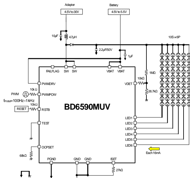
Figure 21. 10series \times 6Parallel, LED current 16mA, Switching frequency 1250kHz setting example Power control PWM application
