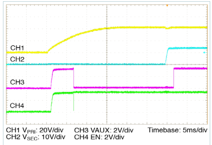
Figure 17 — Start up from application of V_{PRI\_DC} = 42V , 20% I_{SEC\_OUT\_DG} , 100% C_{SEC\_OUT\_EXT}
