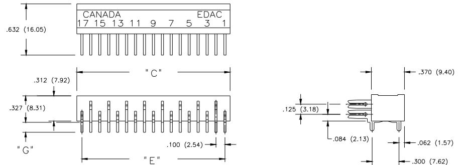
422 SERIES CONNECTOR
