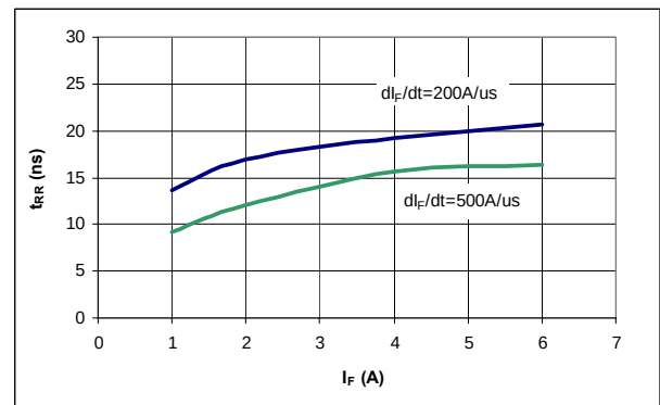
Figure 8. t_{RR} vs I_F at T_J = 125^\circ\text{C}
