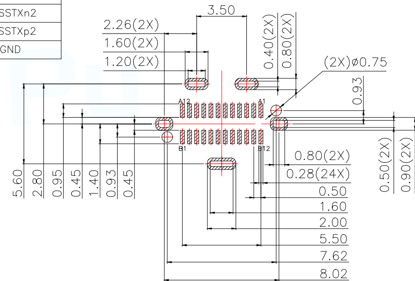
RECOMMENDED PCB LAYOUT(TOP VIEW) THICKNESS 0.8±0.10MM;DEFAULT TOLERANCE:±0.05
