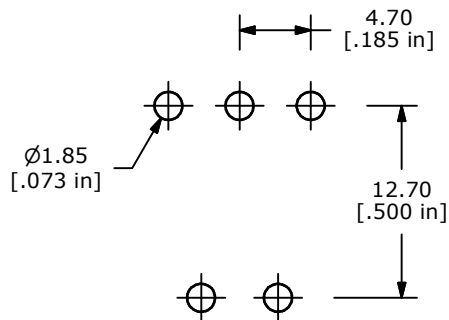
P.C. MOUNTING
