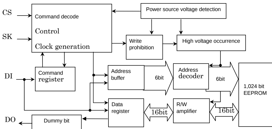
Figure 3. Block Diagram
