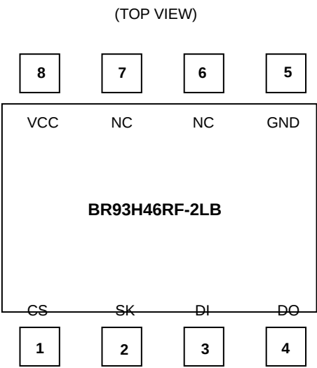
Figure 2. Pin Configuration
