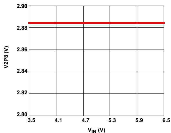
FIGURE 9. V2P8 OUTPUT vs INPUT VOLTAGE
