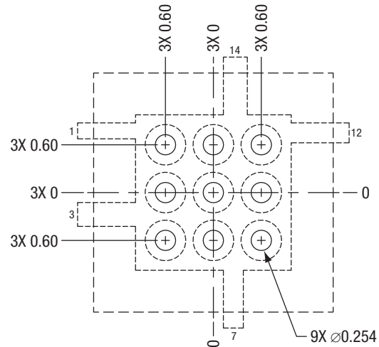
Via Pattern (Note 1)
