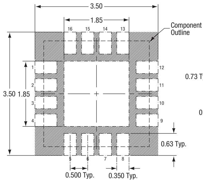
Solder Mask Pattern (Note 2)
