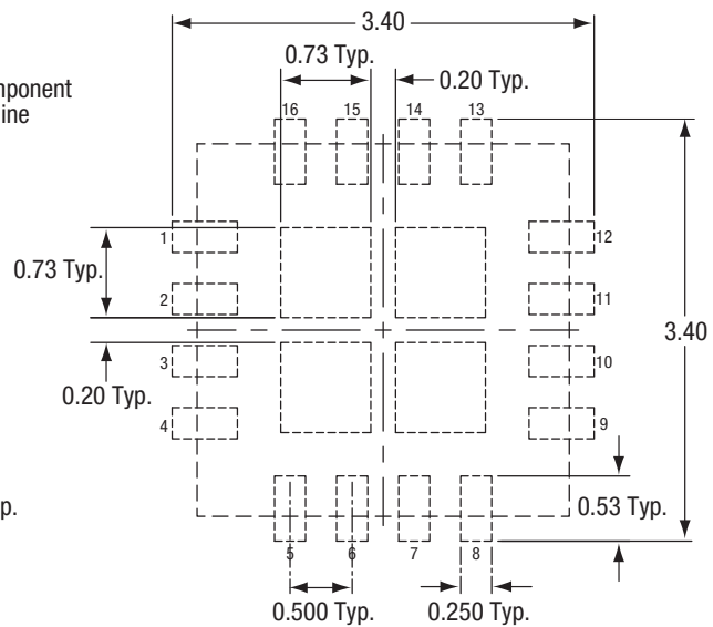
Stencil Pattern (Note 3)
