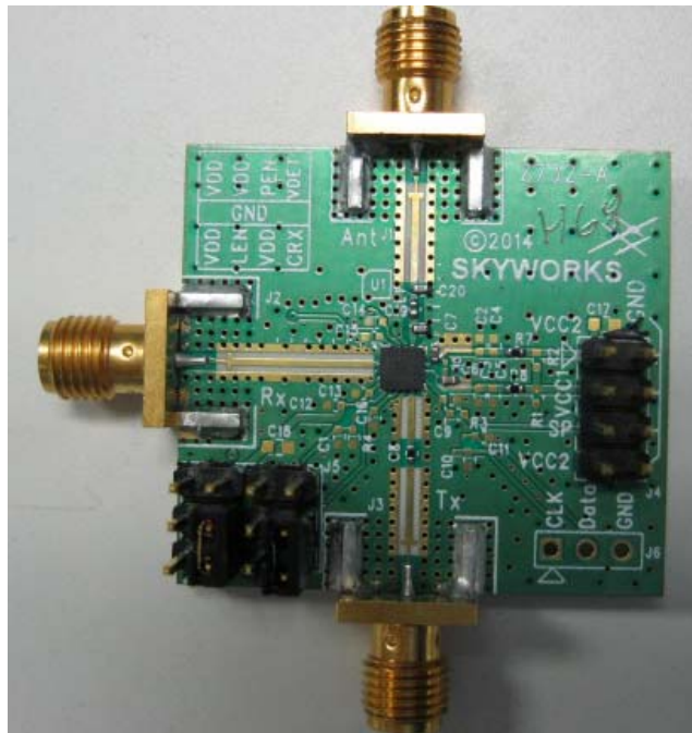
Figure 4. SKY85712-11 Evaluation Board
