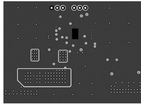
Mid-Layer 1
