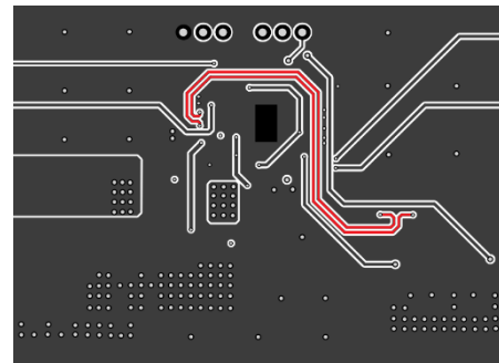
Mid-Layer 2
