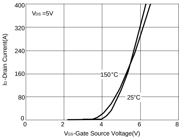
Figure 3: Transfer Characteristics
