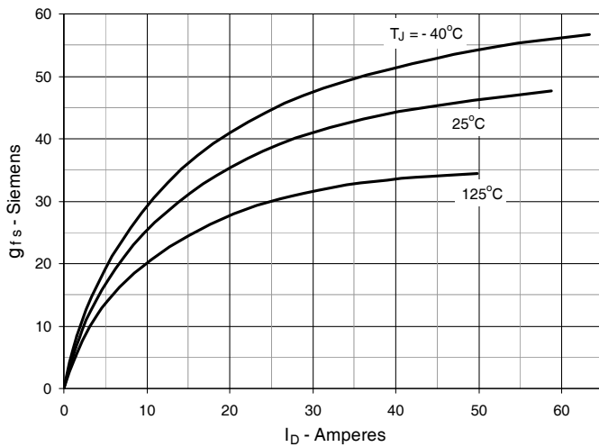
Fig. 9. Transconductance
