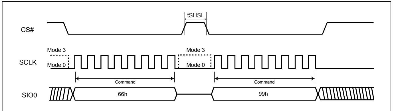
Figure 39. Reset Sequence
