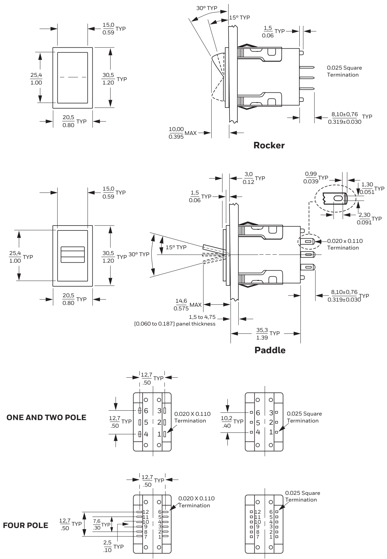
Figure 15. AML23 and AML24 Series Dimensions, mm [in] or mm/in
