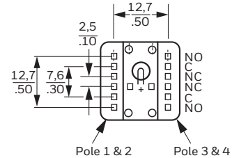
0.025 in Square Termination
