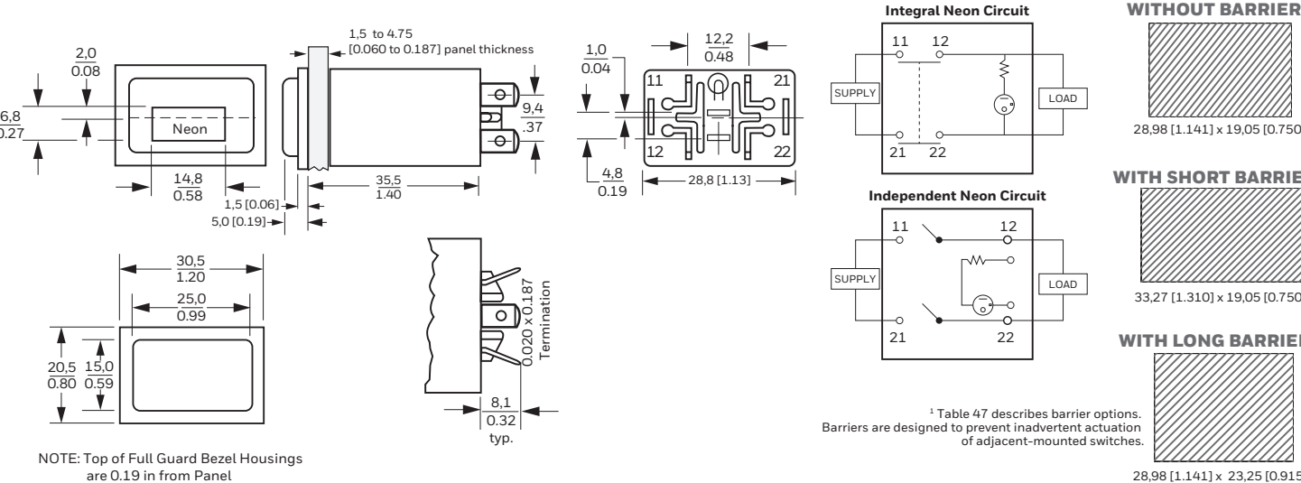
Figure 9. AML32 Series Dimensions mm [in] or mm/in
