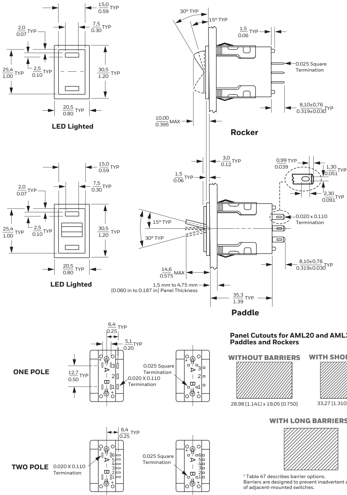
Figure 37. AML25 and AML26 Series Dimensions, mm [in] or mm/in
