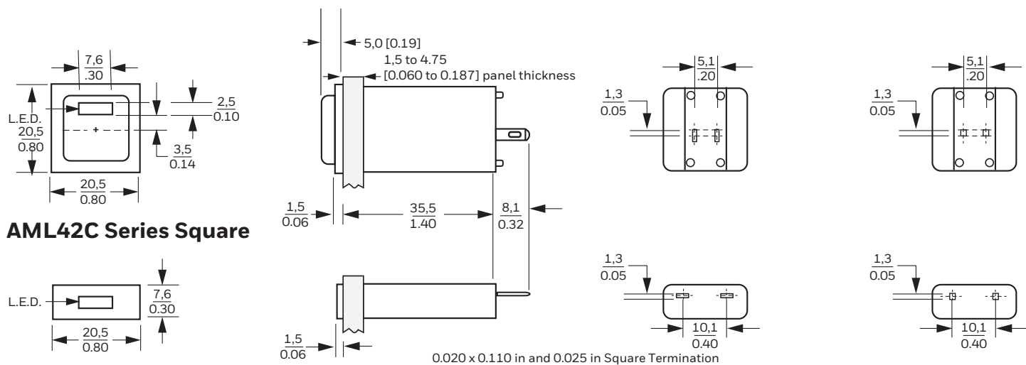
Figure 48. AML42 Series Dimensions, mm [in] or mm/in
