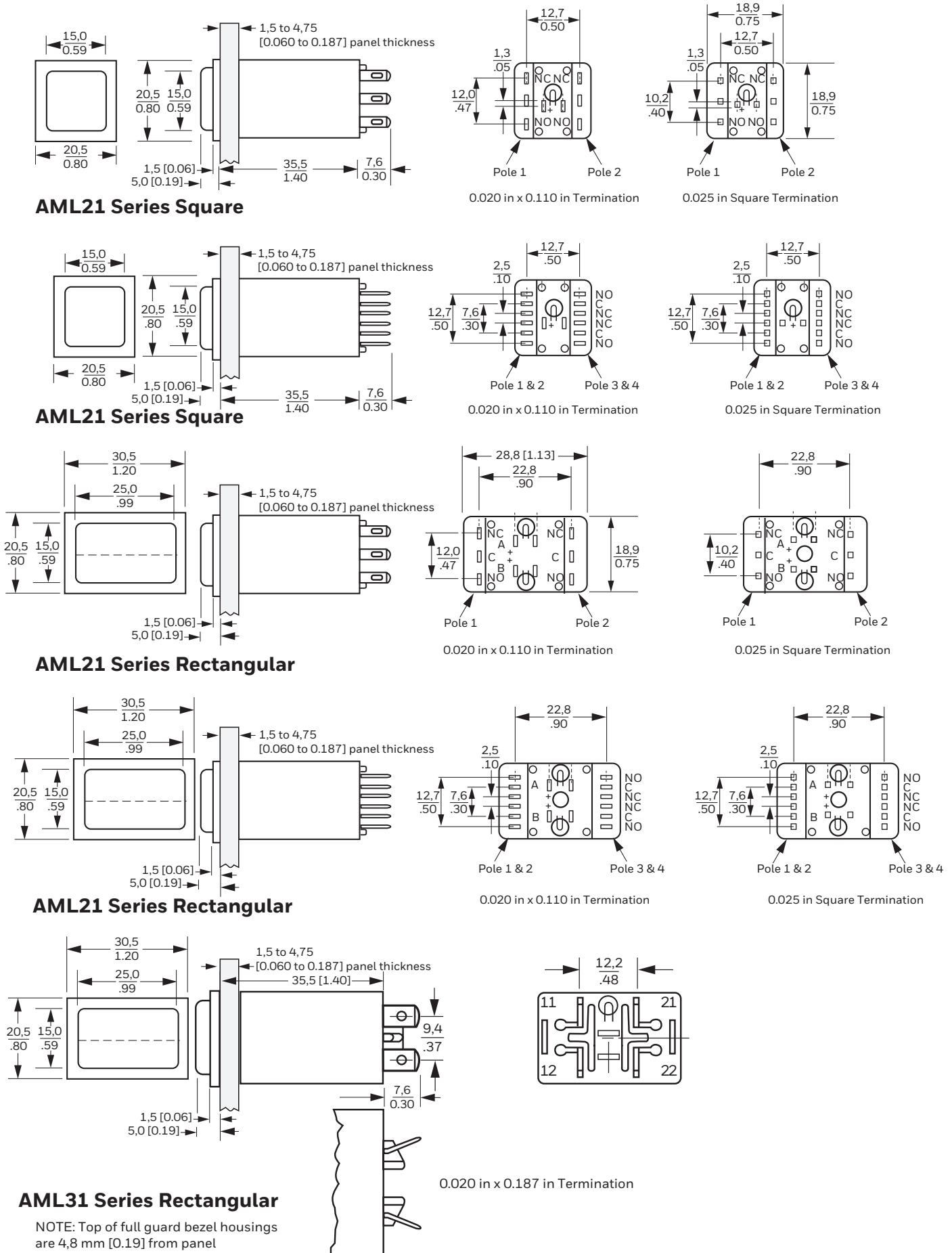
Figure 1. AML21 and AML31 Series Dimensions, mm [in] or mm/in
