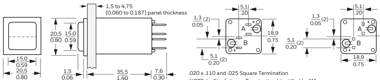
Figure 44. AML41 Series Dimensions, mm [in] or mm/in
