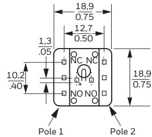
0.025 in Square Termination
