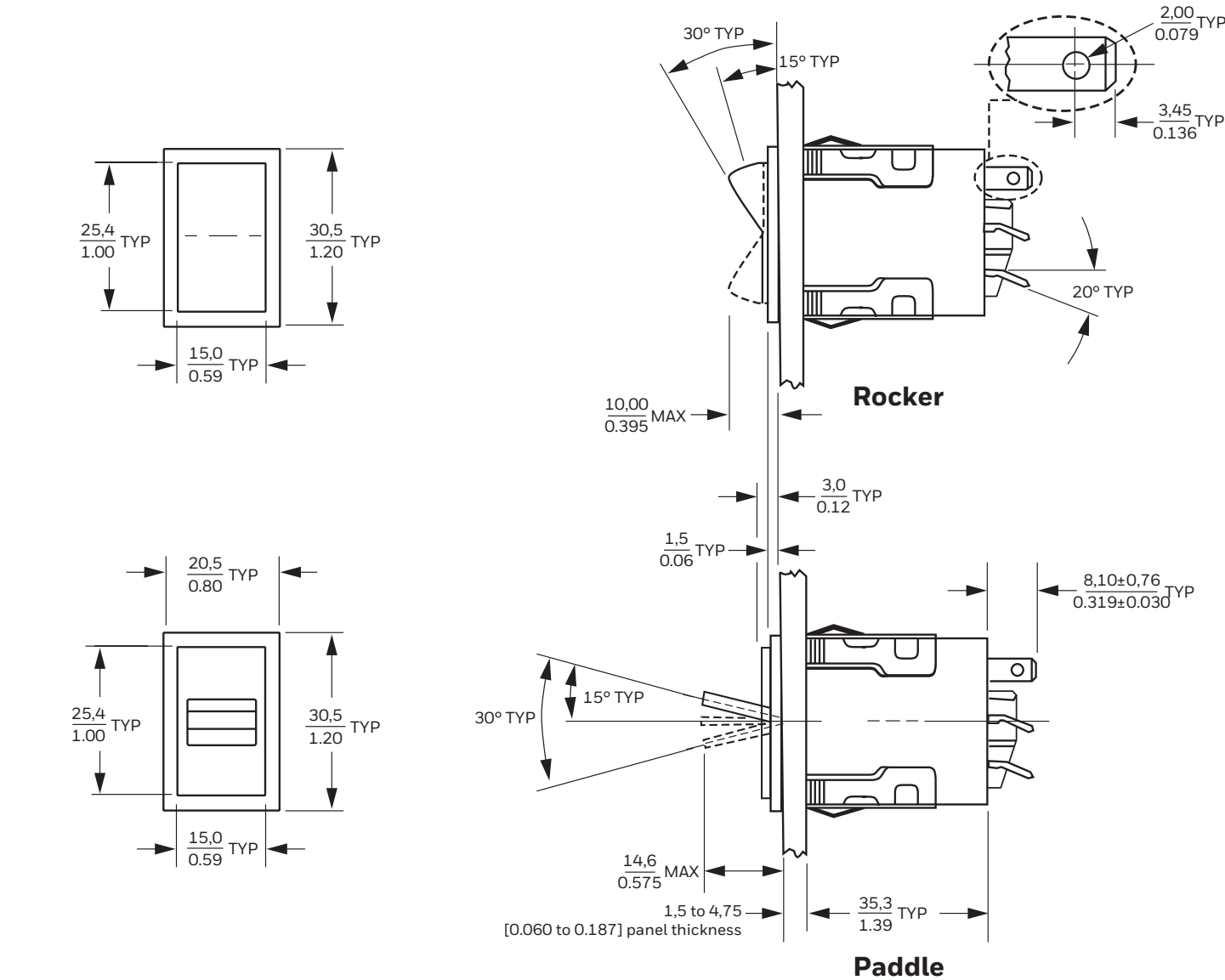
Figure 28. AML33 and AML34 Series Dimensions
