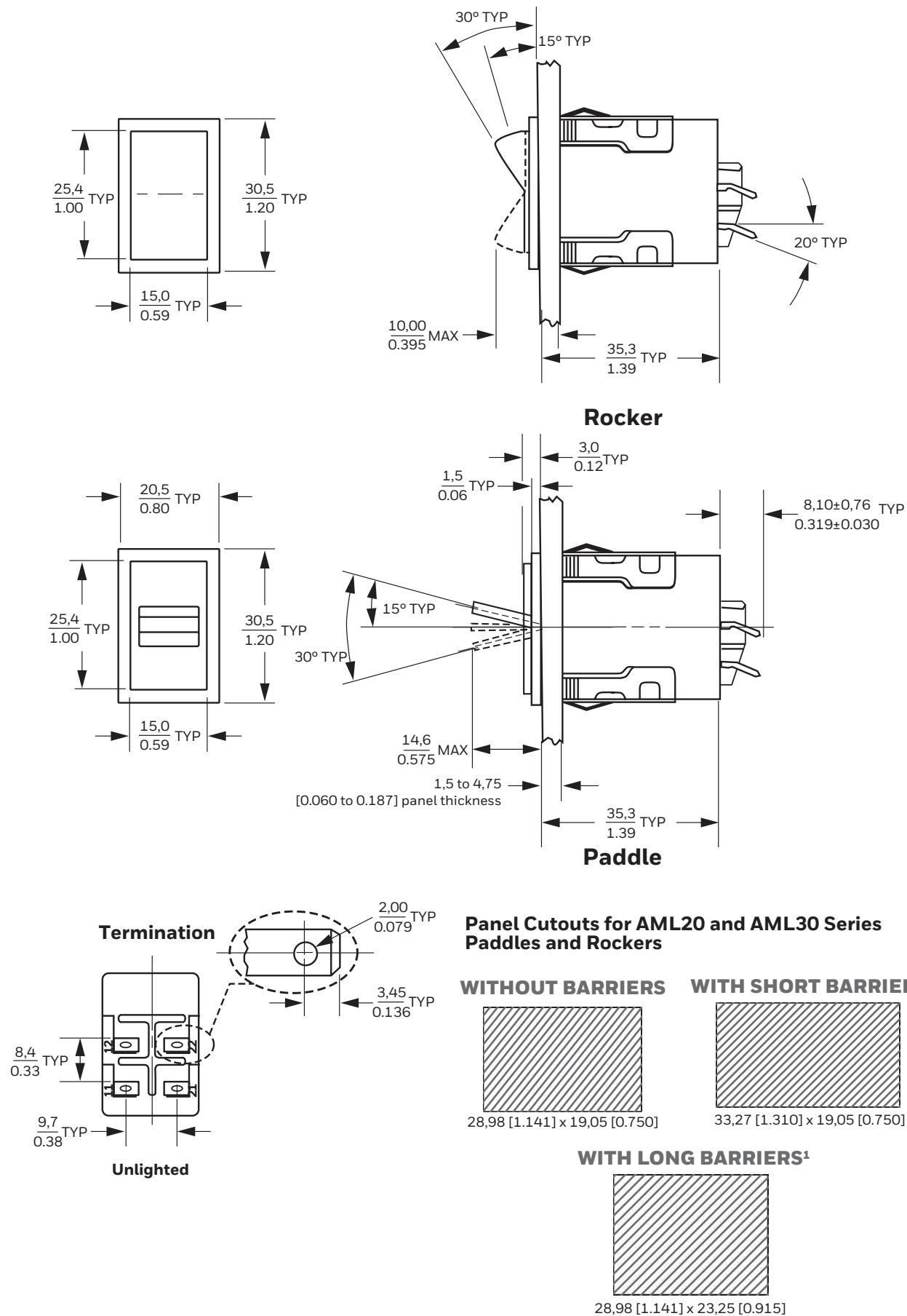
Figure 16. AML33 and AML34 Series Dimensions, mm[in] or mm/in
