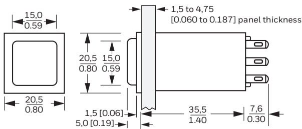
AML21 Series Square
