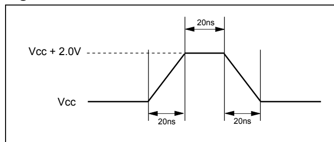
Figure 38. Maximum Positive Overshoot
