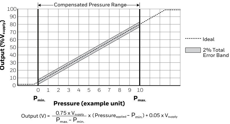
FIGURE 2. TRANSFER FUNCTION LIMITS
