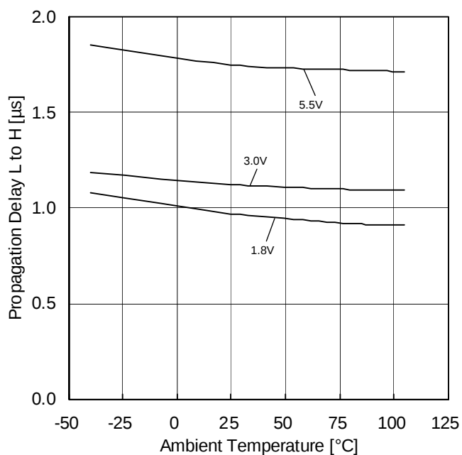
Figure 21. Propagation Delay L to H vs Ambient Temperature ( C_L=15\text{pF} , I_N=-1.5\text{V} 100mV Overdrive)
