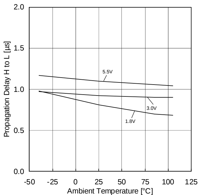
Figure 22. Propagation Delay H to L vs Ambient Temperature ( C_L=15\text{pF} , I_N=-1.5\text{V} 100mV Overdrive)
