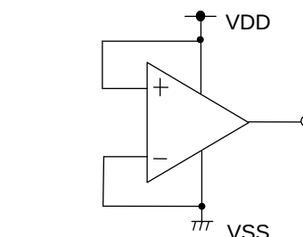
Figure 27. Example of Application Circuit for Unused Comparator
