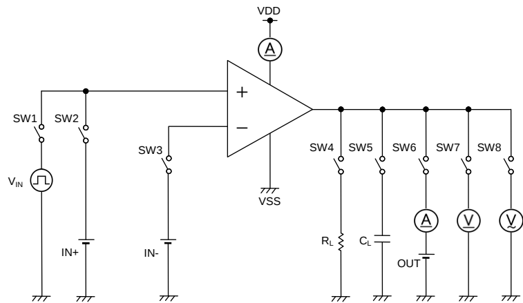
Figure 24. Test Circuit 2
