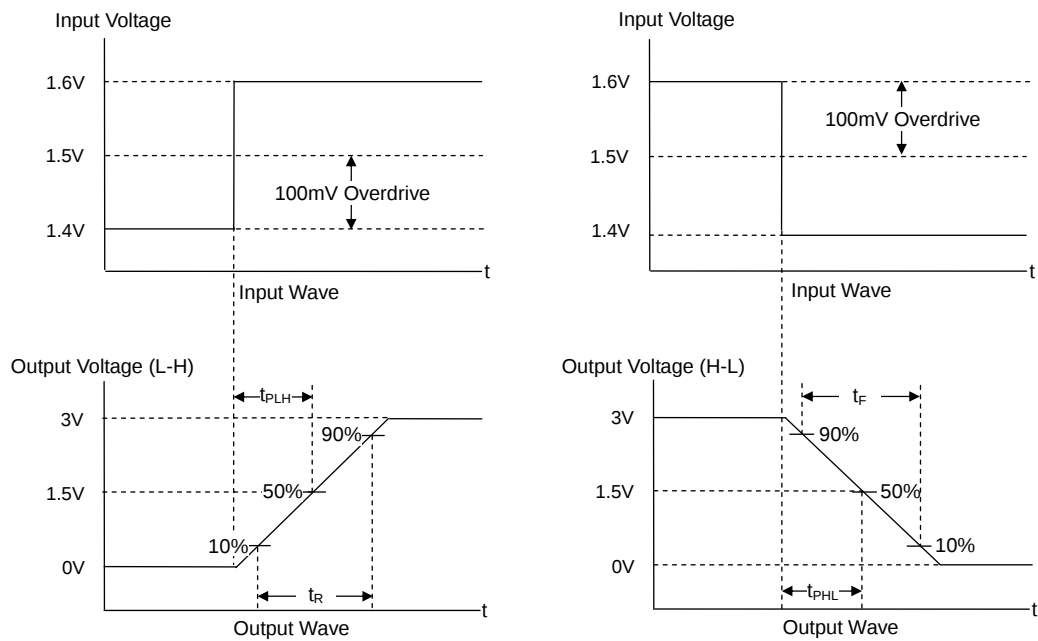
Figure 25. Response Time Input and Output Wave
