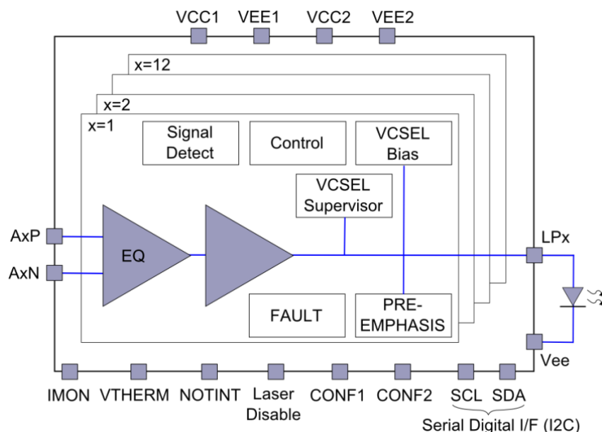
Figure 1: Device diagram
