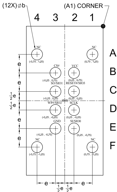
BOTTOM VIEW
