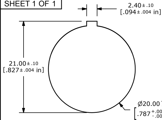
PANEL CUTOUT
