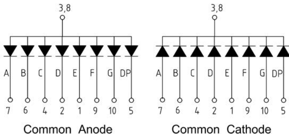
Figure 2: Circuit Diagram
