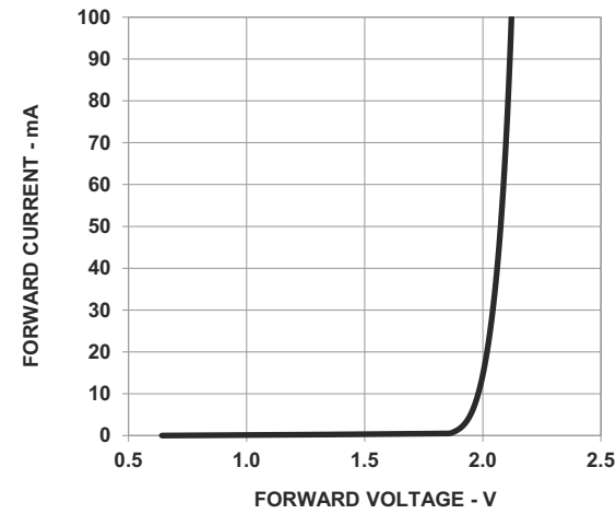
Figure 7: Forward Voltage vs. Current
