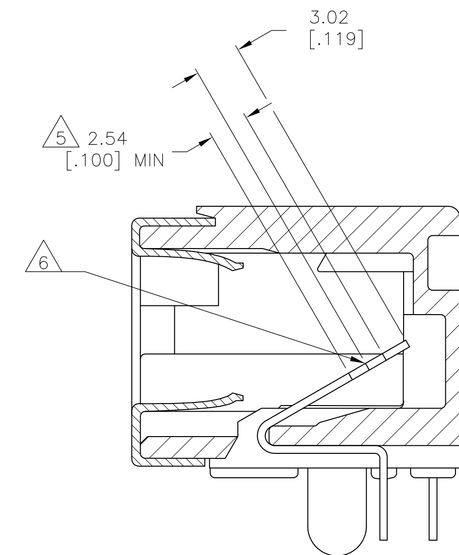
SECTION J-J
