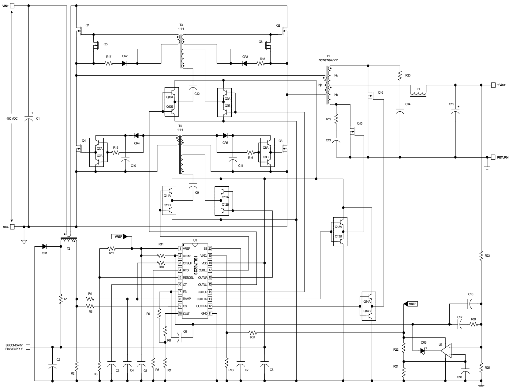
FIGURE 5. HIGH VOLTAGE INPUT SECONDARY SIDE CONTROL ZVS FULL-BRIDGE CONVERTER
