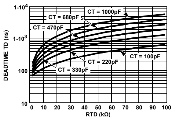
FIGURE 8. DEADTIME (DT) vs CAPACITANCE
