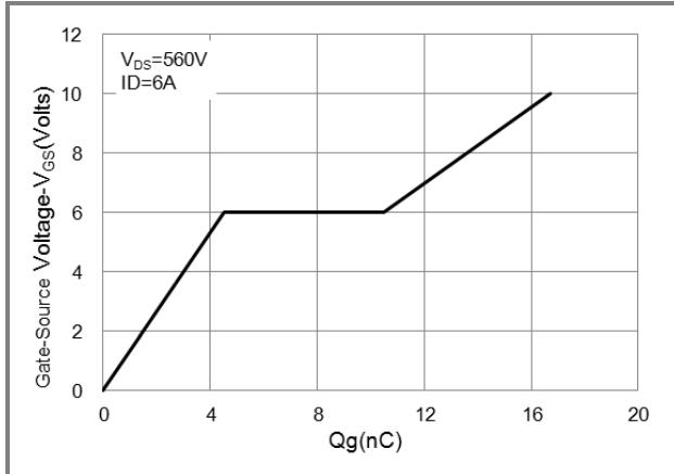
Fig.7 Gate Charge
