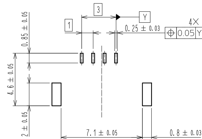
RECOMMENDED STENCIL PATTERN (RECOMMENDED STENCIL THICKNESS: t=0.12)
