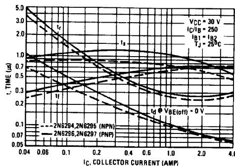
FIGURE 3 – SWITCHING TIMES
