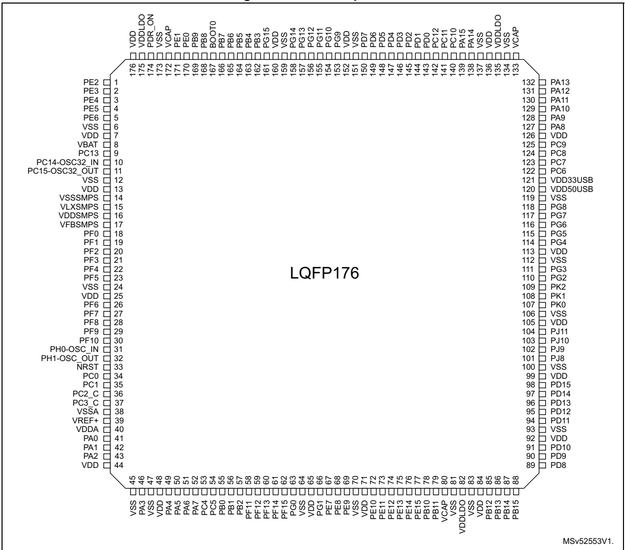
Figure 9. LQFP176 pinout
