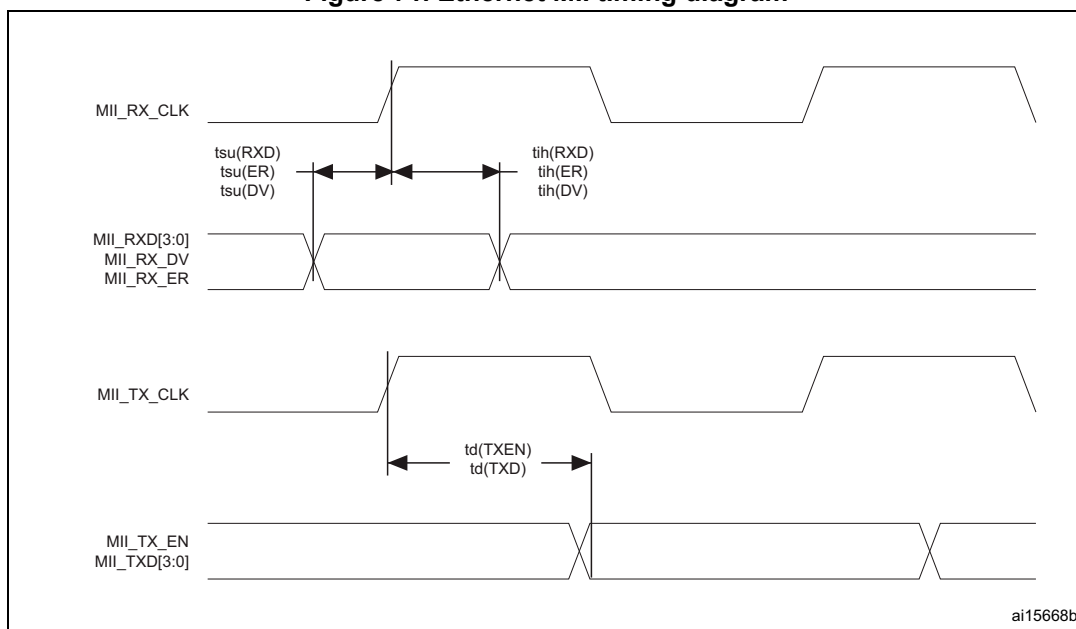
Figure 71. Ethernet MII timing diagram
