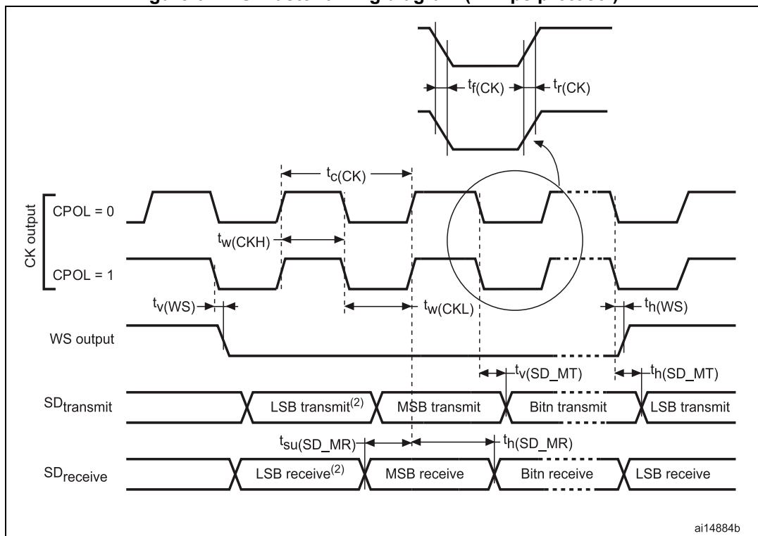
Figure 61. I²S master timing diagram (Philips protocol) (1)
