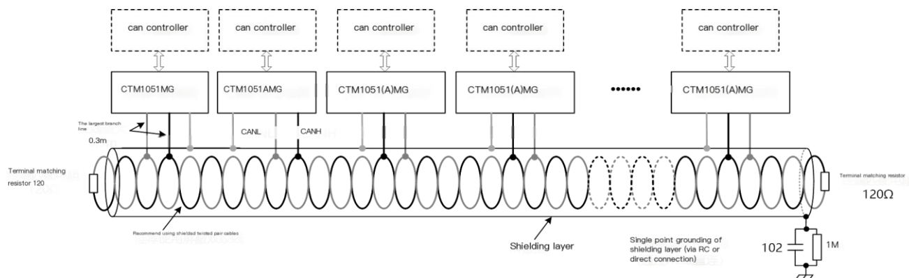
Figure 3. Schematic diagram of typical network connection for a single CAN Bus
