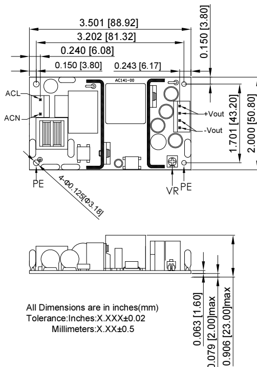
CFM20XXS Series
