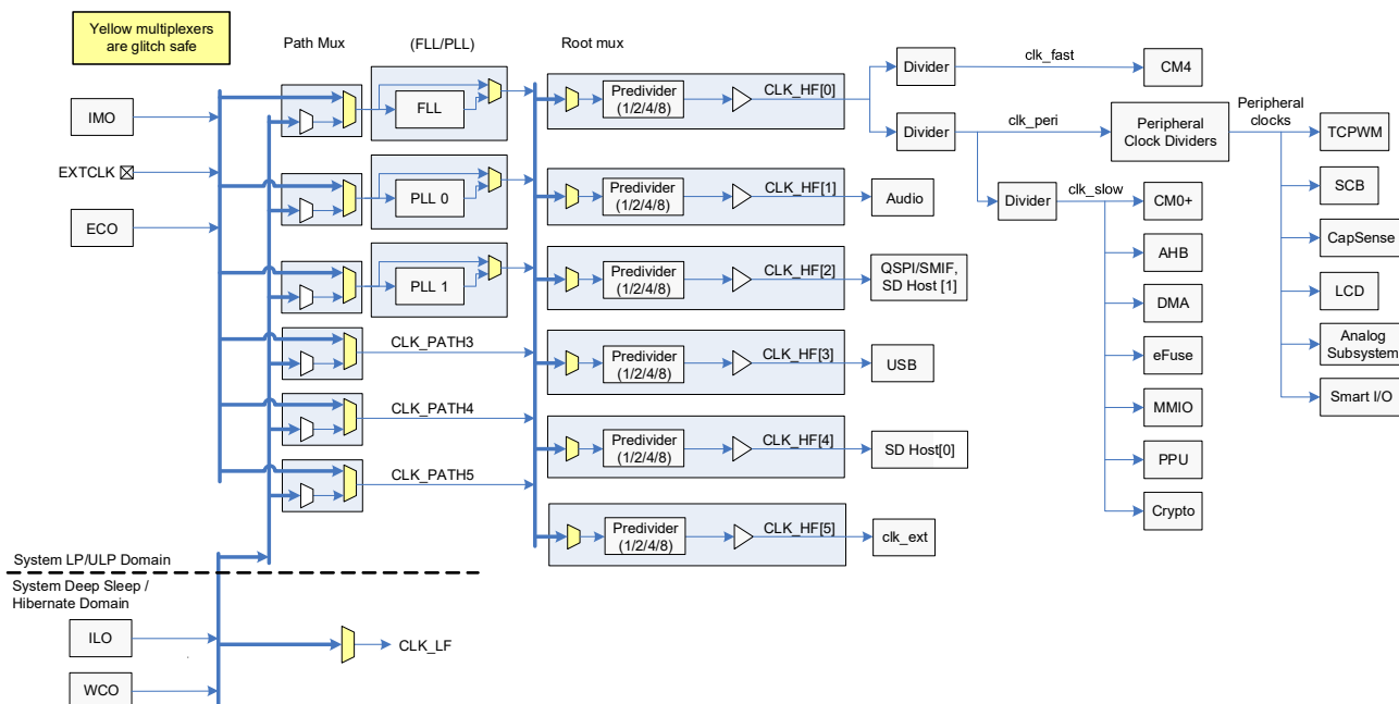
Figure 3. Clocking Diagram
