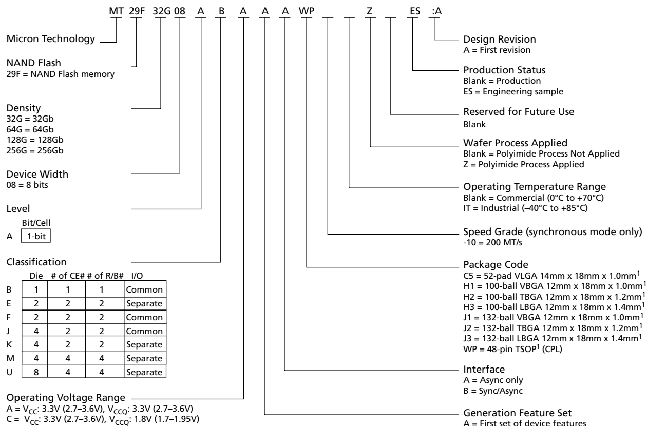
Figure 1: Part Numbering
