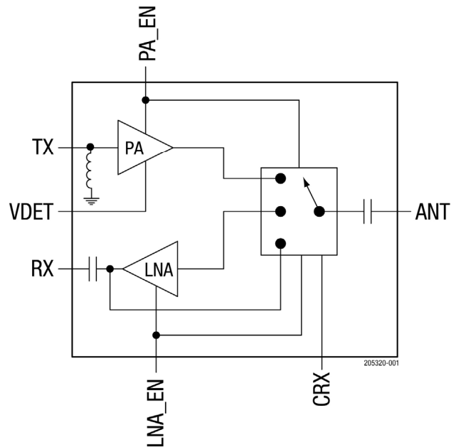
Figure 1. SKY85726-11 Block Diagram
