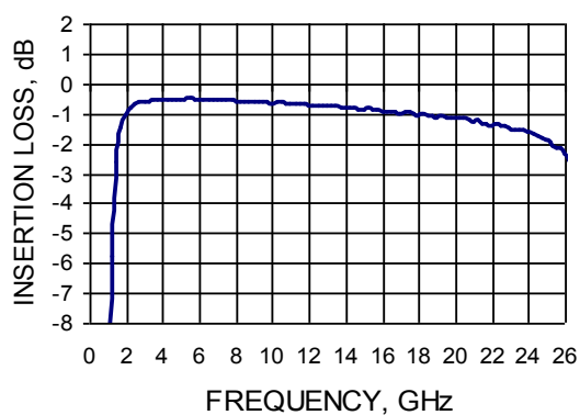
INSERTION LOSS vs FREQUENCY MA4SW310B-1
