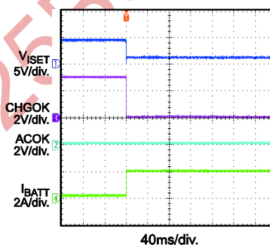
Indication @ Charge On/Off
