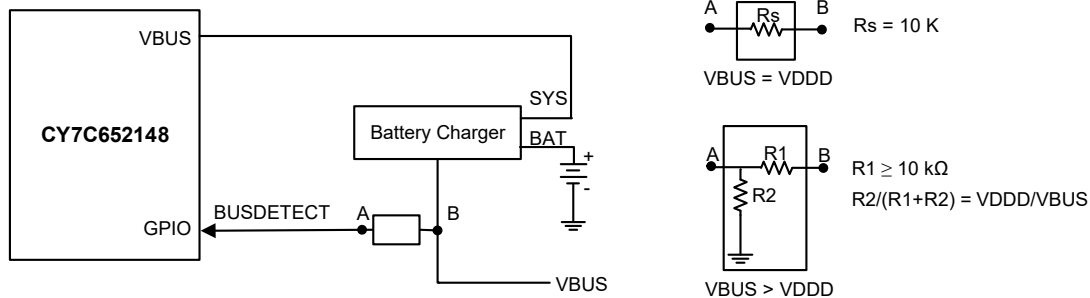
Figure 9. 9 V Tolerant
