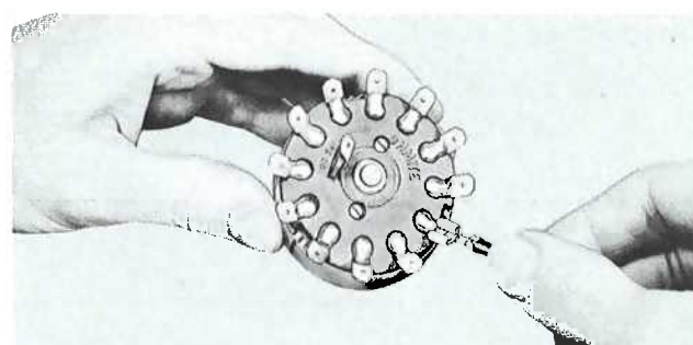
Fig. 210—Model 212 Tap Switch with Push-on Terminals.
