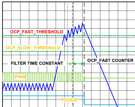
FIGURE 22. OCP_FAST
